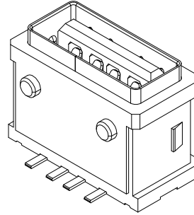
3D VIEW
