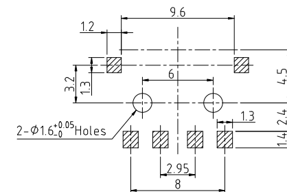
P.C.B.MOUNTING DETAIL
