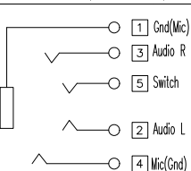
SCHEMATIC (PLUG OUT)
