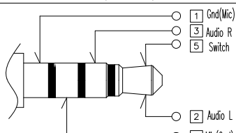
SCHEMATIC (PLUG IN)
