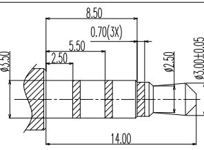
(ø3.50mm 4 POLE PLUG DETAIL DRAWING)
