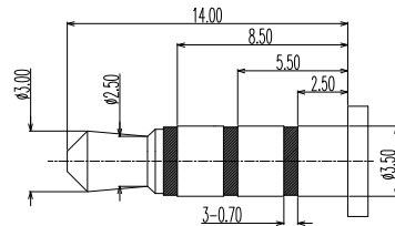
(ø3.50mm 4 POLE PLUG )
