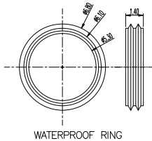
WATERPROOF RING
