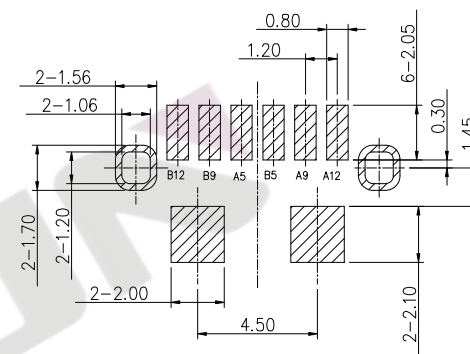
RECOMMENDED P.C.B LAYOUT TOP VIEW (TOLRANCE: \pm 0.05 )
