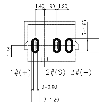
RECOMMENDED P.C.B LAYOUT TOP VIEW (TOLRANCE:±0.05)
